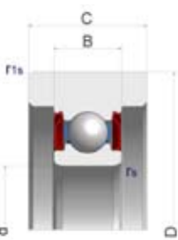
*5 - Special ball bearing covered by metal shields and with extended outer ring, with radial clearance Gr 0,005 to 0,020 mm.
