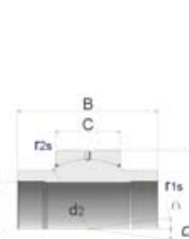
*8 - Special spherical bearing with extended inner ring with radial clearance Gr 0,20 to 0,35 mm.
